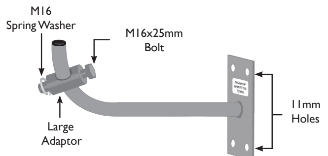
HEAVY DUTY ZINC PLATED J-BRACKET
