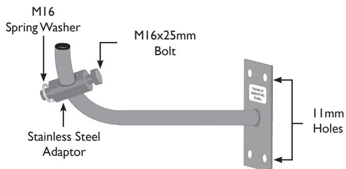
ELECTRO-POLISHED STAINLESS STEEL HEAVY DUTY J-BRACKET
