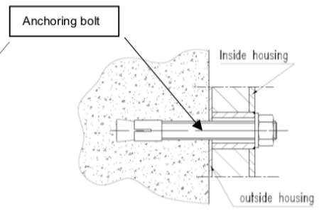
Anchoring through the rear wall Model Grade 3 and 4
