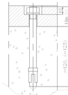
Anchoring through the bottom
