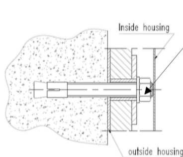
Anchoring through the rear wall Model Grade 0, 1 & 2
