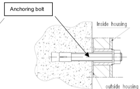
Anchoring through the rear wall Model Grade 3 and 4
