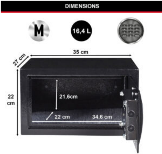
X055ML_DIMENSIONS
