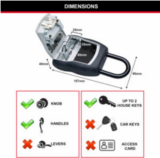
5400EURD_DIMENSIONS
