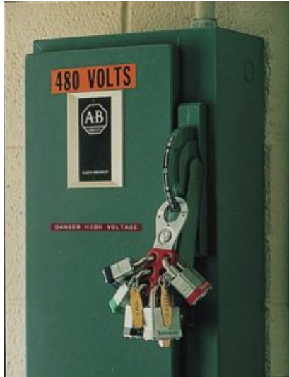
Scissor Type Safety Lockout Hasp
